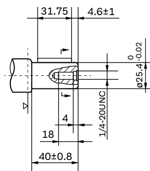
Shaft: Cylindrical shaft ø25.4 Parallel key 6.35x6.35x31.75
