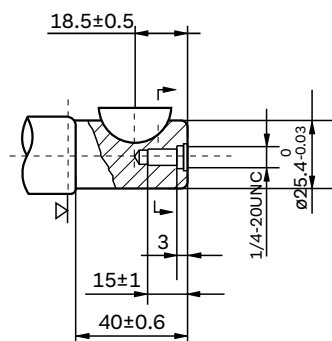
Shaft K: Cylindrical shaft Ø25.4 Woodruff key Ø25.4x6.35
