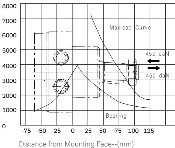
VNKG2 for W# Mounting Side Load-(daN)
