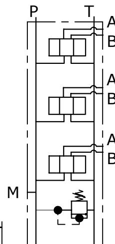
Schema idraulico Hydraulic diagram
