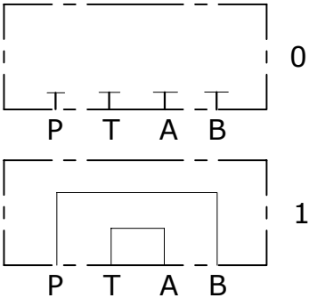
Schema idraulico Hydraulic diagram
