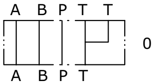
Schema idraulico Hydraulic diagram
