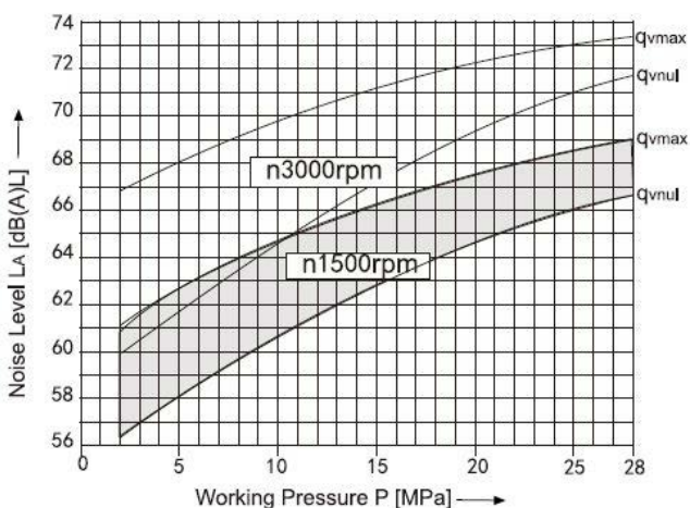
Size 100/110
