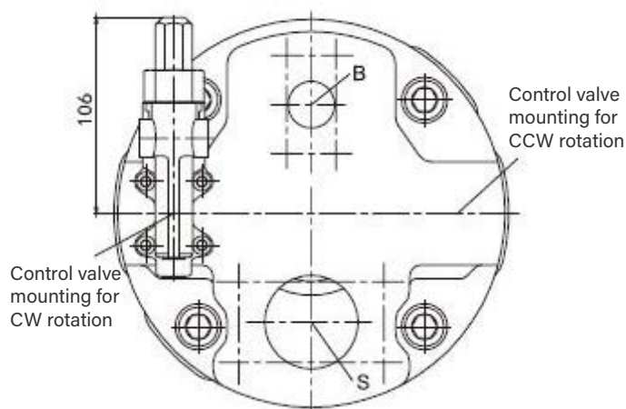
Detail K
