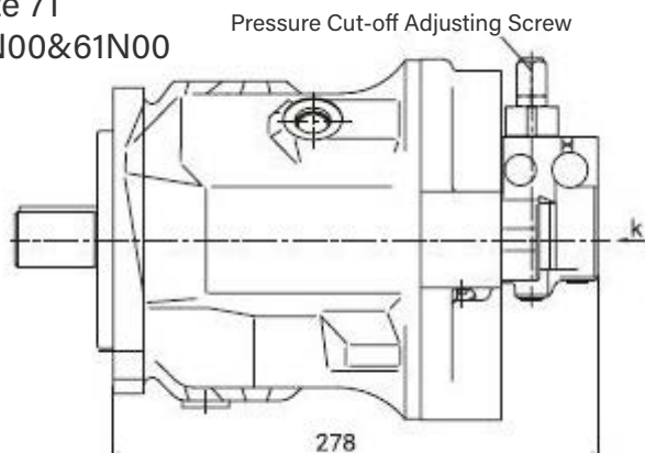
Pressure Cut-off Adjusting Screw
