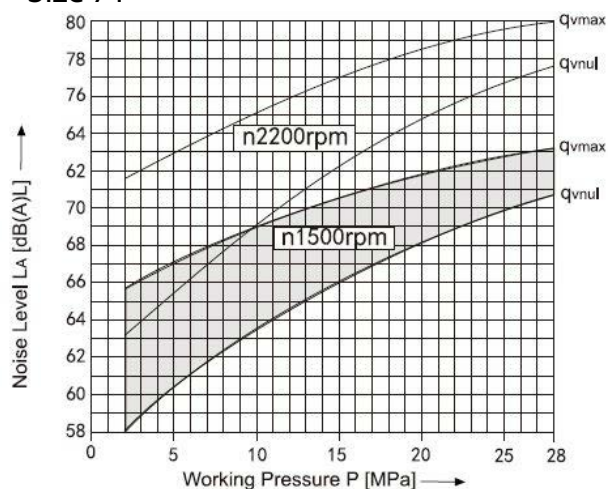
Size 140
