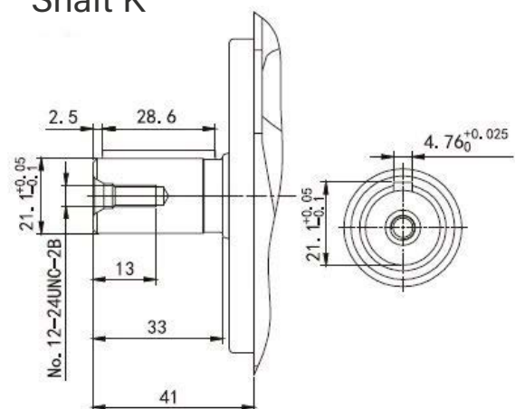
Shaft K
