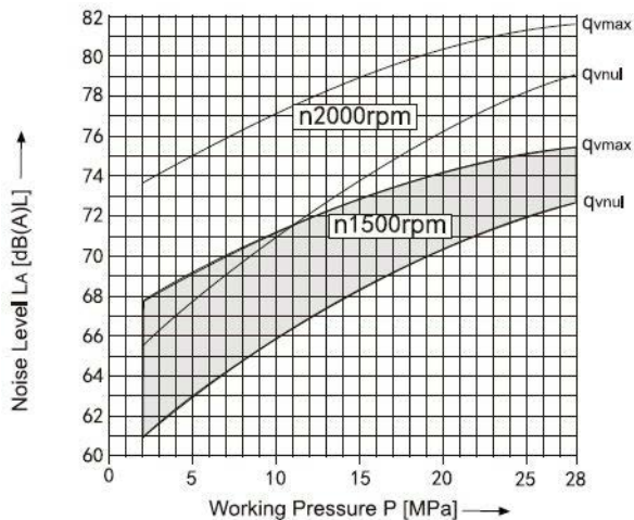
Size 100/110
