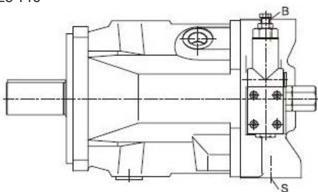
Control valve mounting for CCW rotation
