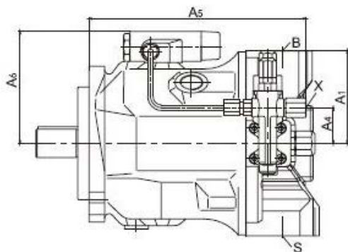
Size 71 11N00&61N00
