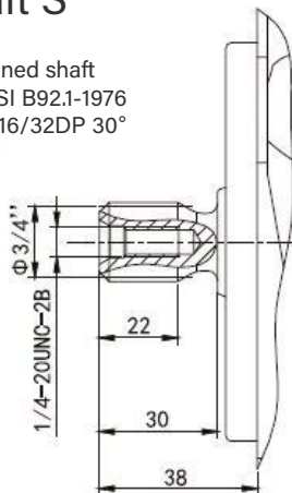
Shaft S
