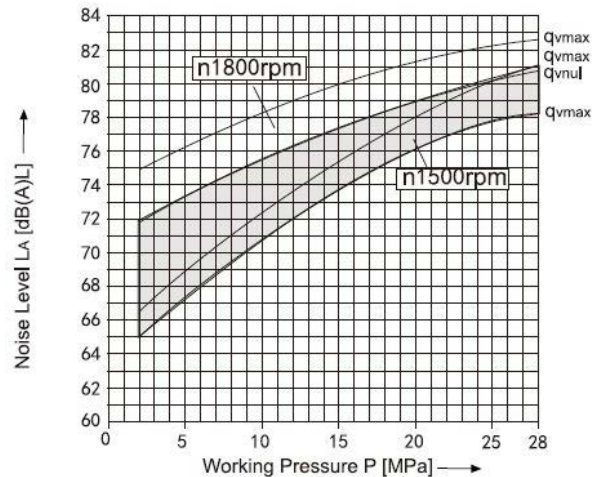
Size 140
