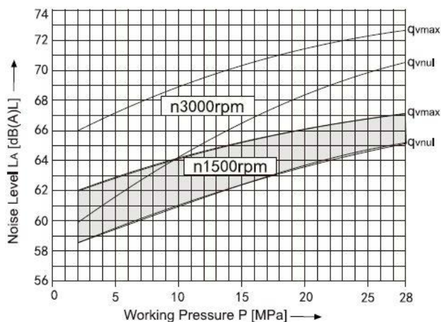
Size 45
