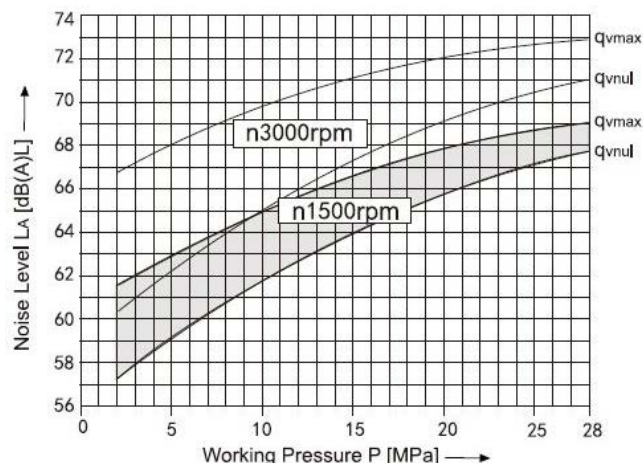
Size 71
