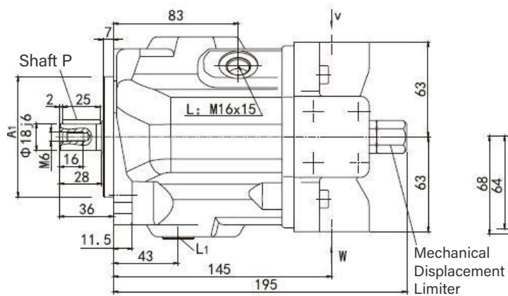
Shaft P
