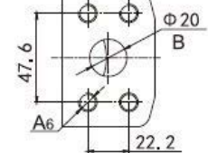
Detail V
