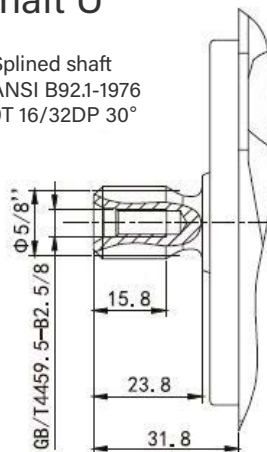
Shaft U
