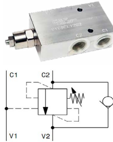
OVERCENTER SIMPLE PILOTAJE INTERNO 350 BAR CUERPO ALUMINIO SINGLE INTERNAL PILOT OPERATED LOAD CONTR.VAL.350 BAR ALUMINIUM BODY VALVE D'ÉQUILIBRAGE SIMPLE PILOTAGE INTERNE 350 BAR CORPS ALUMINIUM
