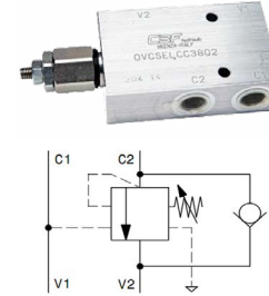
OVERCENTER SIMPLE PILOTAJE INTERNO CENTRO CERRADO 350 BAR CUERPO ALUMINIO SINGLE INTERNAL PILOT OPERATED LOAD CONTR.VAL. CLOSED CENTER 350 BAR ALUMINIUM BODY VALVE D'ÉQUILIBRAGE SIMPLE PILOTAGE INTERNE CENTRE FERME 350 BAR CORPS ALUMINIUM
