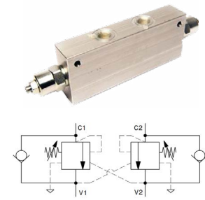
OVERCENTER DOBLE CENTRO CERRADO 350 BAR CUERPO ALUMINIO DOUBL LOAD CONTR.VAL. CLOSED CENTER 350 BAR ALUMINIUM BODY VALVE D'ÉQUILIBRAGE DOUBLE CENTRE FERME 350 BAR CORPS ALUMINIUM
