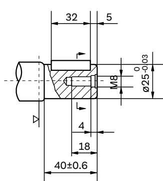
Shaft J: Cylindrical shaft \varnothing 25 Parallel key 7 \times 32
