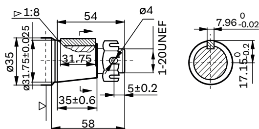
Shaft T3:
