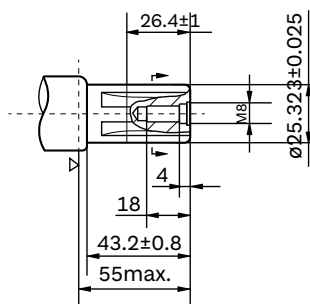
Shaft E: Splined SAE 6B
