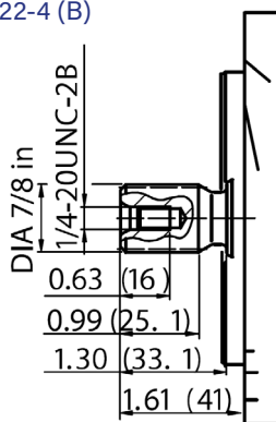
S Splined shaft 7/8 in in 13T 16/32 DP SAE J744-22-4 (B)
