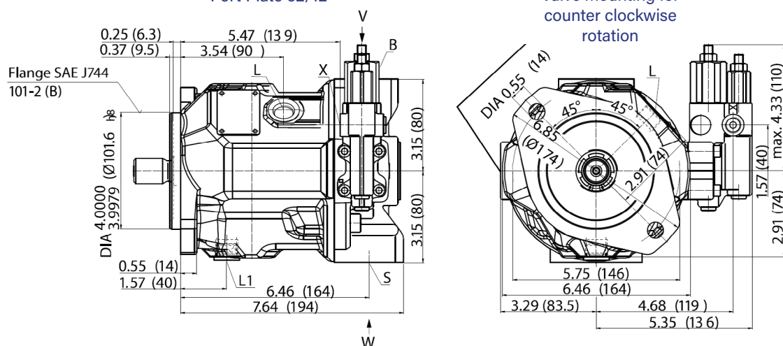
Port Plate 62/12
