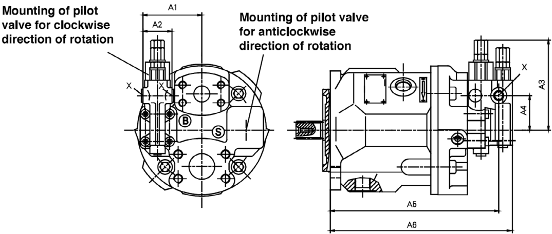
Service Ports at Rear; Models 61N00 and 11N00
