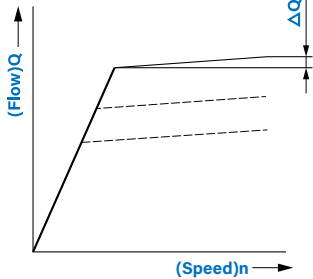
Static characteristic at variable speed
