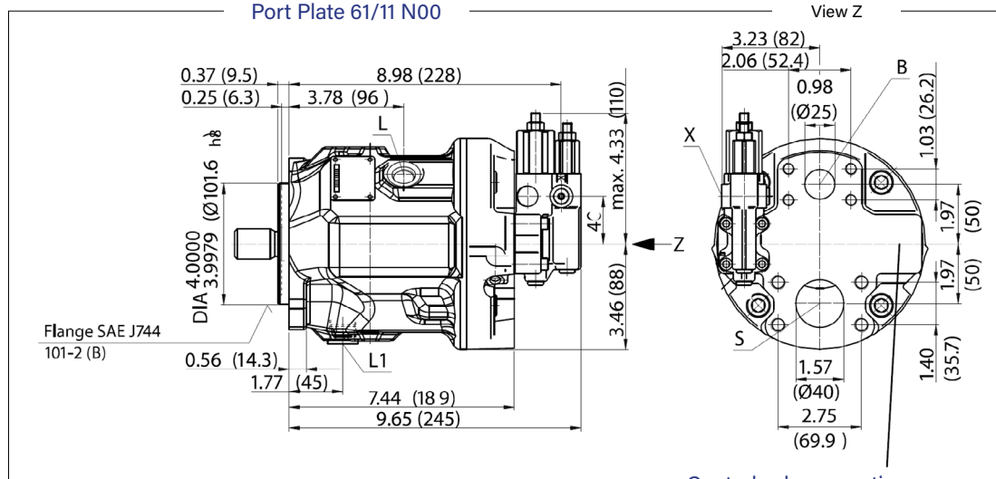
Port Plate 61/11 N00
